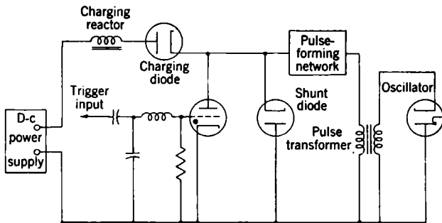
FIG. 8-40.—A typical hydrogen-thyratron pulser circuit.
